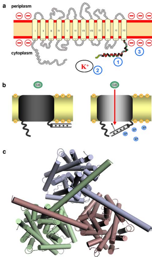
Fig. 5 Structure-function correlation of BetP activation. a Elements of BetP activity control including the C-terminal, regulatory domain I, the cytoplasmic concentration of K^+ 2, and negative membrane surface charges 3. b Mechanistic concept of BetP activation involving the elements described in a . In this concept, in the resting state, the C-terminal domain is interacting with the adjacent membrane. Upon activation by an increase in cytoplasmic K^+ , the C-terminal domain switches its conformation, interacts with not yet defined regions of BetP, and as a result, BetP actively transports glycine betaine. c Structural elements of the functionally active BetP trimer derived from the X-ray structure (Ressl et al. 2009; Krämer and Ziegler 2009). The three individual monomers of BetP are differently color-coded. The C-terminal domains, which are recognized as long helices lying on the cytoplasmic surface of the adjacent BetP monomers, are not fully resolved in the X-ray structure (Ressl et al. 2009), their conformation was modeled in accordance with other biochemical data (Krämer and Ziegler 2009)
