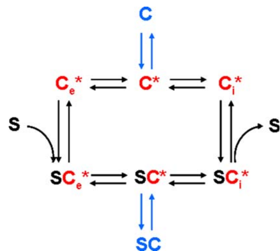
Fig. 4 Catalytic cycle and activation cycle of BetP. In the activation cycle, BetP alternates between the inactive ( C ) and the active state ( C^* ). The shift from the inactive to the active state may be triggered by the cytoplasmic K^+ concentration and by the membrane surface charge (see text). The catalytic cycle of BetP in the active state involves several conformational states, with the substrate binding site either exposed to the outside ( C_e^* ) or the inside ( C_i^* ), as well as the transition, or occluded state ( C^* ), respectively
