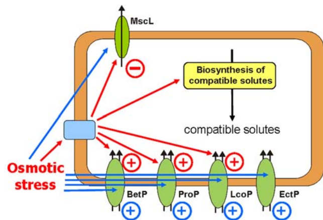
Fig. 1 Stimulus perception and signal transduction in response to hypo- and hyperosmotic stress in C. glutamicum . Osmotic stress leads to regulation both on the level of transcription (red arrows) and protein activity (blue arrows) of uptake systems of compatible solutes (BetP, EctP, ProP, LcoP), mechanosensitive solute efflux systems (MscL, MscS), as well as biosynthesis pathways for compatible solutes
